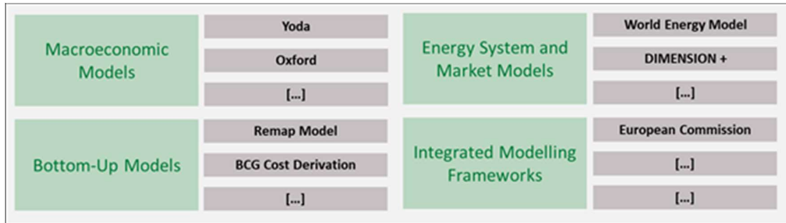
Figure 2 - Model Families
